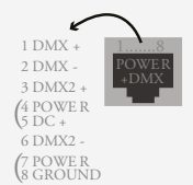
POWER+DMX WITH THE RJ45 C ABLE
